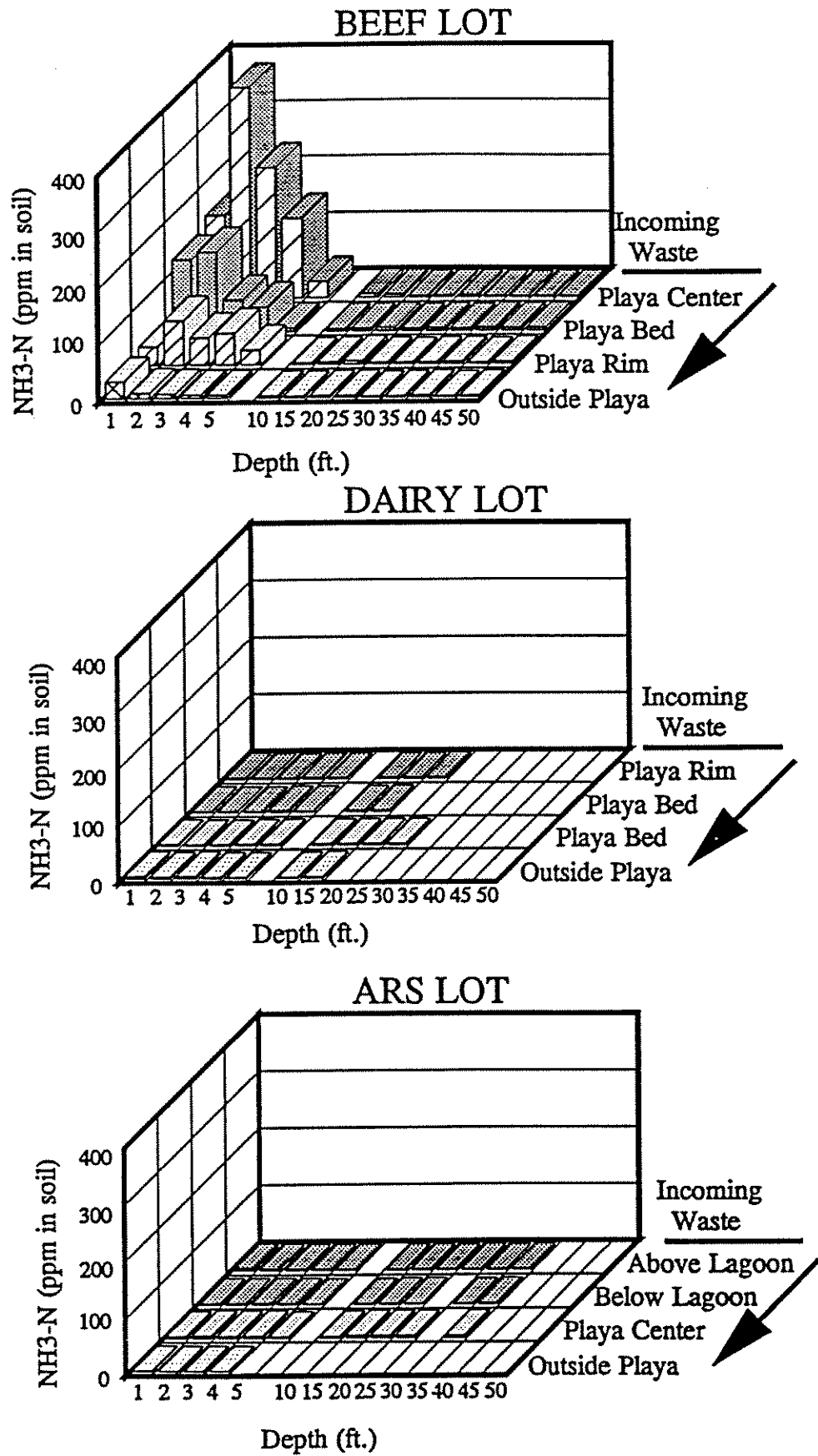
Figure 7. Ammonium-N concentrations in soil profiles at drill sites.
