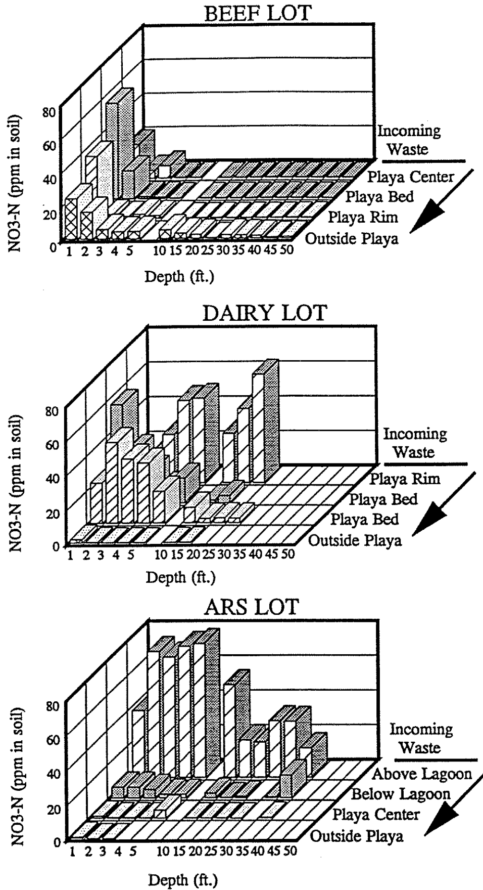
Figure 6. Nitrate-N concentrations in soil profiles at drill sites.
