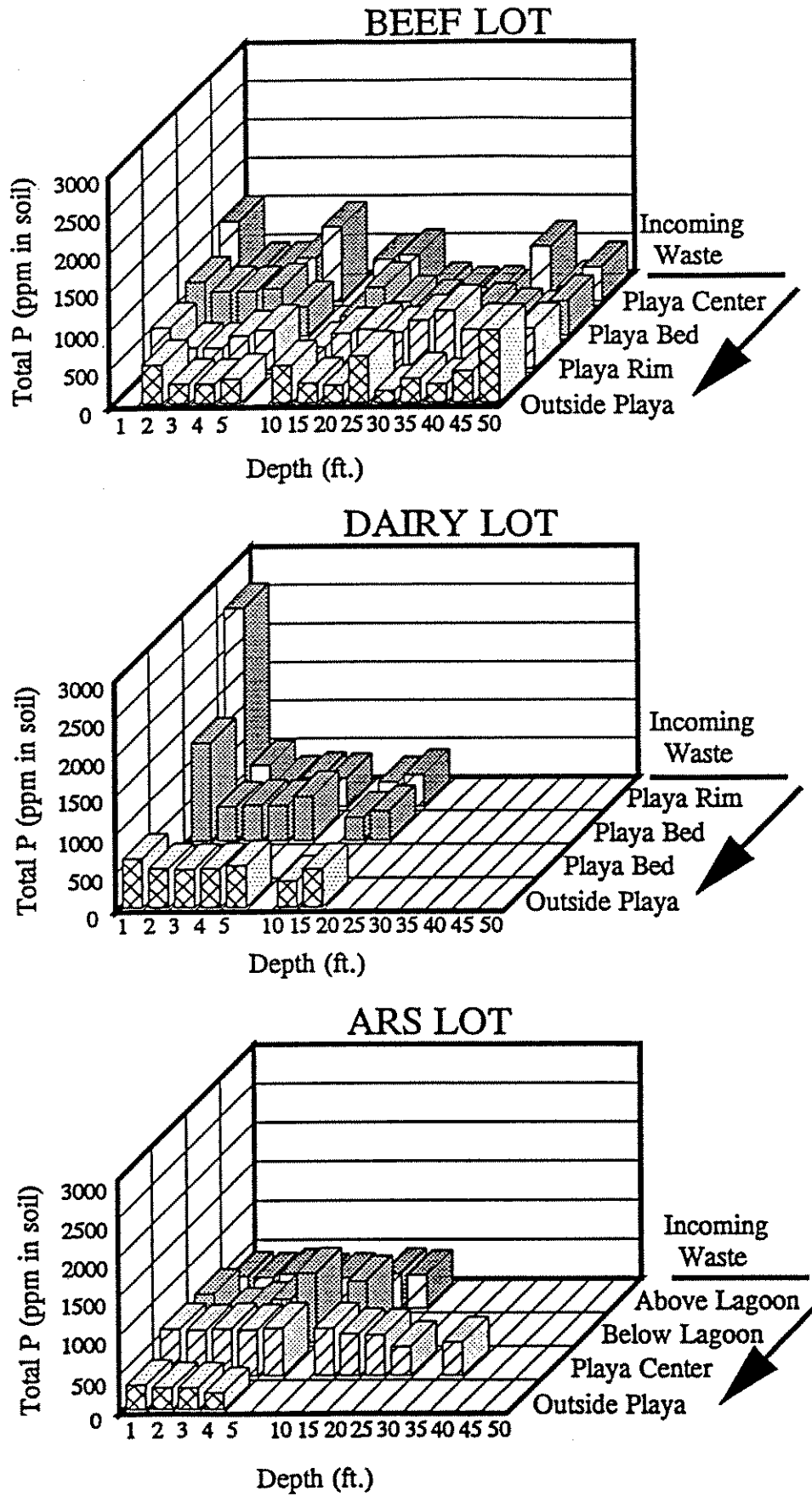
Figure 9. Total P concentrations in soil profiles at drill sites.
