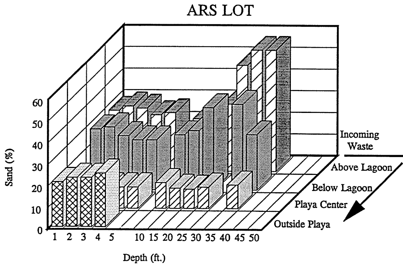
Figure 13. Sand concentrations in soil profiles at drill sites.
