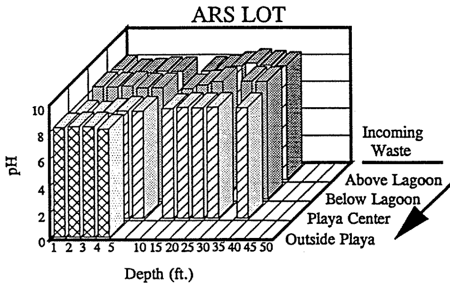
Figure 12. Values of pH in soil profiles at drill sites.
