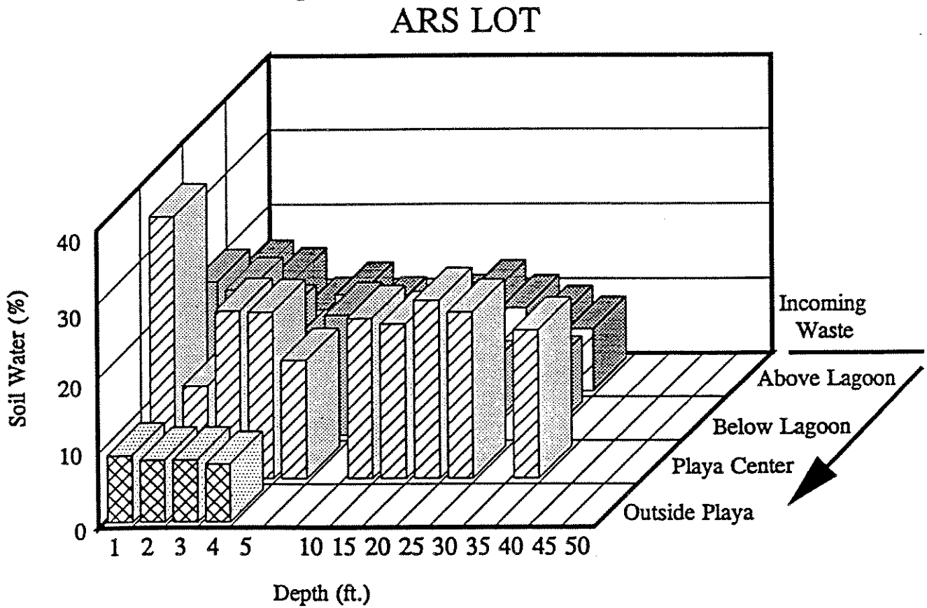
Figure 16. Water contents in soil profiles at drill sites.
